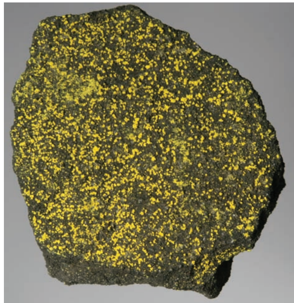
FIGURE 16. Massive black coffinite (ideally USiO_4 ), with a yellow coating of the secondary uranyl sulfate zippelite [K_3(UO_2)_4(SO_4)_2O_3(OH) \cdot 3H_2O] , formed in the sediment-hosted Grants mineral belt, Section 35 Mine, Jurassic Morrison Formation, New Mexico. Photo courtesy of Robert Lauf. Specimen is 7 cm wide; individual masses of zippelite are up to ~1 mm.
