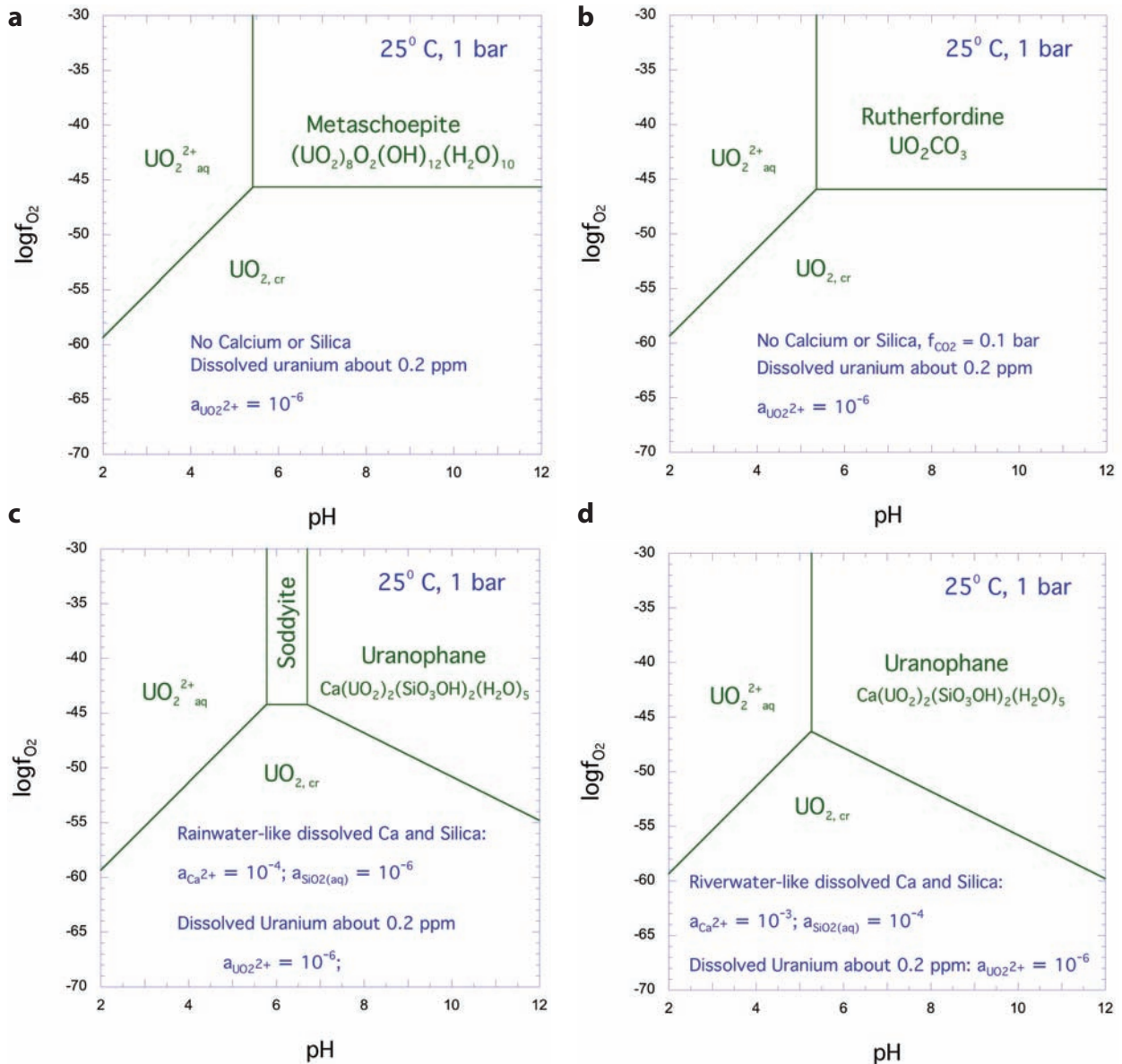
FIGURE 4. Calculated \log f_{\text{O}_2} -pH diagrams illustrating the stability of uraninite ( \text{UO}_{2,\text{cr}} ) relative to a variety of uranyl minerals at 25 °C and 1 bar. The solubilities of the minerals are expressed relative to an aqueous activity for (\text{UO}_2)_{(\text{aq})}^{2+} of 10^{-6} . Aqueous complexing of (\text{UO}_2)_{(\text{aq})}^{2+} (for example, with carbonate or phosphate) could significantly expand the field of (\text{UO}_2)_{(\text{aq})}^{2+} relative to the minerals. Calculations are based on data of Shock et al. (1997a, 1997b), Chen et al. (1999), and Finch and Murakami (1999).
