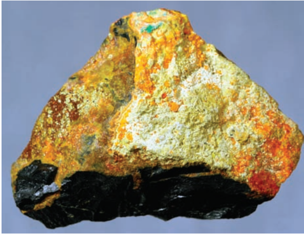
FIGURE 7. Auto-oxidation leads to the formation of Pb-uranium secondary minerals. Here reddish orange fourmarierite [Pb_{1-x}O_{3-2x}(UO_2)_4(OH)_{4+2x} \cdot 4H_2O] and bright orange vandendriesscheite [Pb_{1.6}(UO_2)_{10}O_6(OH)_{11} \cdot 11H_2O] , along with pale yellow rutherfordine [(UO_2)(CO_3)] , form a crust of secondary minerals on massive primary uraninite ( UO_2 ) from Shinkolobwe, Congo. Photo courtesy of Robert Lauf. Specimen is 5 cm wide.
