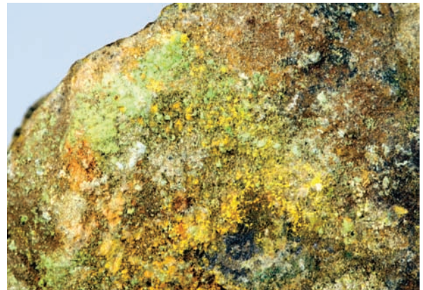
FIGURE 13. Uranyl sulfate minerals (~20 known species) only form where sulfides are being oxidized to produce aqueous SO_4 ions, coupled with evaporation. Here pale green johannite [Cu(UO_2)_2(SO_4)_2(OH)_2 \cdot 8H_2O] occurs with yellow zippeite [K_3(UO_2)_4(SO_4)_2O_3(OH) \cdot 3H_2O] in a specimen from Roughton Consols, Bodmin Moor, Cornwall, England. Photo courtesy of Robert Lauf. Field of view is 3 cm wide.
