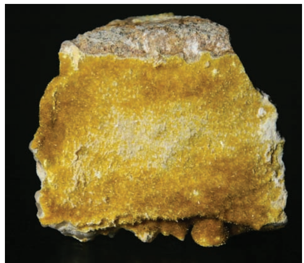
FIGURE 14. The uranyl silicates uranophane and \beta -uranophane [Ca(UO_2)_2(SiO_3OH)_2 \cdot 5H_2O] are the most common U^{6+} minerals. Here \beta -uranophane needles coat a matrix surface (specimen from Rössing, Namibia). Photo courtesy of Robert Lauf. Specimen is ~10 cm wide.
