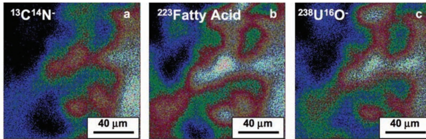
◀ FIGURE 18. Data of Fayek et al. (2005) reveal that some microbes couple enzymatic metabolic acetate oxidation to the reduction of aqueous uranyl cations ( \text{U}^{6+}\text{O}_2 ) 2+ to uraninite. These micro-SIMS images of (a) ^{13}\text{C}^{14}\text{N} molecules and (b) fatty acids that mark the location of Geobacter biofilms match the location of ^{238}\text{U}^{16}\text{O} (c). These images thus show that where there are no bacteria, there is also no uranium oxide. Courtesy of Mostafa Fayek.
