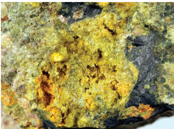
FIGURE 12. Many of the ~30 known uranyl carbonate species are found only as weathering products of mine tailings, while others occur as alteration products of previously formed uranyl carbonates. Here yellow kamotoite-(Y) [Y_2O_4(UO_2)_4(CO_3)_3 \cdot 14H_2O] forms as small crystals on altered uraninite ( UO_2 ). Photo courtesy of Robert Lauf. Field of view is 2.5 cm wide.
