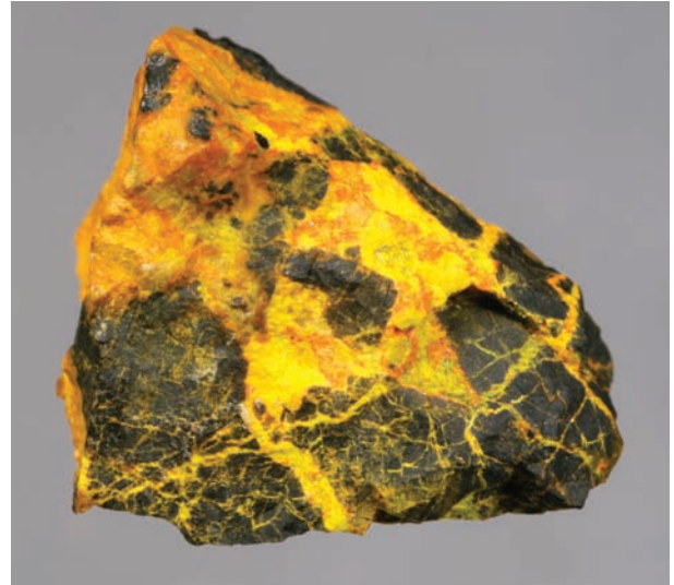
FIGURE 8. Lemon yellow schoepite [(\text{UO}_2)_8\text{O}_2(\text{OH})_{12}\cdot 12\text{H}_2\text{O}] , amber becquerelite [\text{Ca}(\text{UO}_2)_6\text{O}_4(\text{OH})_6\cdot 8\text{H}_2\text{O}] , and orange curite \{\text{Pb}_{3+x}[(\text{UO}_2)_4\text{O}_{4+x}(\text{OH})_{3-x}]_2\cdot 2\text{H}_2\text{O}\} represent progressive alteration of black uraninite ( \text{UO}_2 ) under oxidizing conditions (specimen from Shinkolobwe, Congo). Photo courtesy of Robert Lauf. Specimen is 2 cm in its longest dimension.
