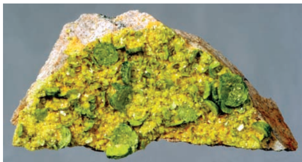
FIGURE 15. An alteration sequence of uranyl oxy-hydroxides to uranyl phosphates is observed to be the last stage of uranyl mineral evolution. Autunite [Ca(UO_2)_2(PO_4)_2 \cdot 10-12(H_2O)] and its many isomorphs are among the most common of the more than 40 species of uranyl phosphates. This specimen is from Luzy, France. Photo courtesy of Robert Lauf. Specimen is 7 cm wide; the largest autunite crystals are ~8 mm across.
