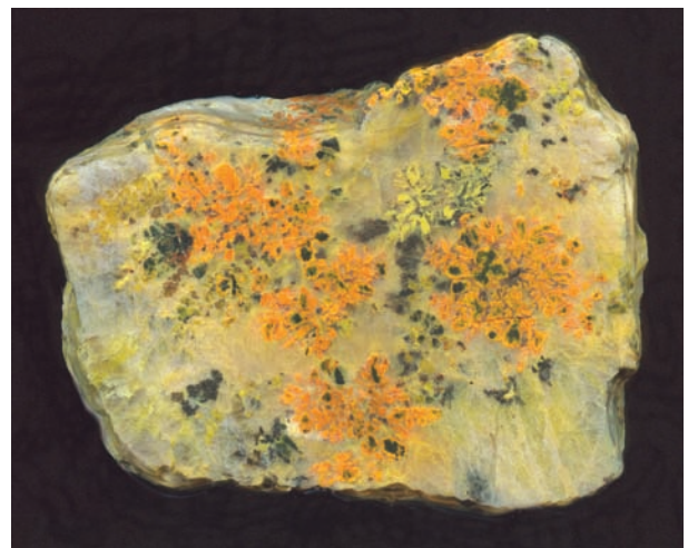
FIGURE 9. Dendritic uraninite mostly altered to “gummite,” which is a mixture of several uranyl minerals, including soddyite, curite, kasolite, uranophane, boltwoodite, and clarkeite (Frondel 1956; Foord et al. 1997). This pegmatitic specimen is from the Ruggles Mine, New Hampshire. Photo courtesy of Robert Lauf. Specimen is 5 cm wide.
