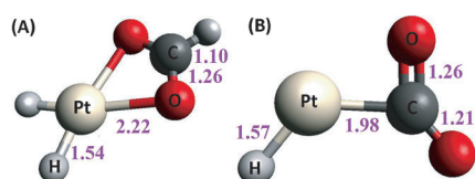
Figure 4. A) Optimized structures of \text{PtCO}_2\text{H}_3^- and B) \text{PtCO}_2\text{H}^- . Bond lengths (Å).
