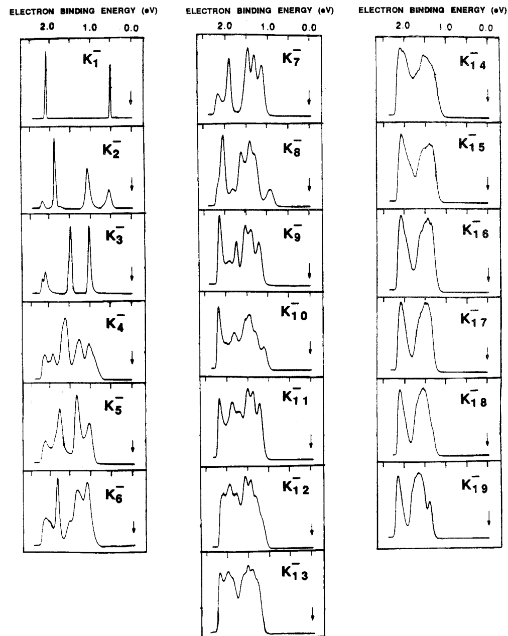
Figure 1. The photoelectron spectra of \text{K}_{1-19}^- recorded with 2.540 eV photons.
