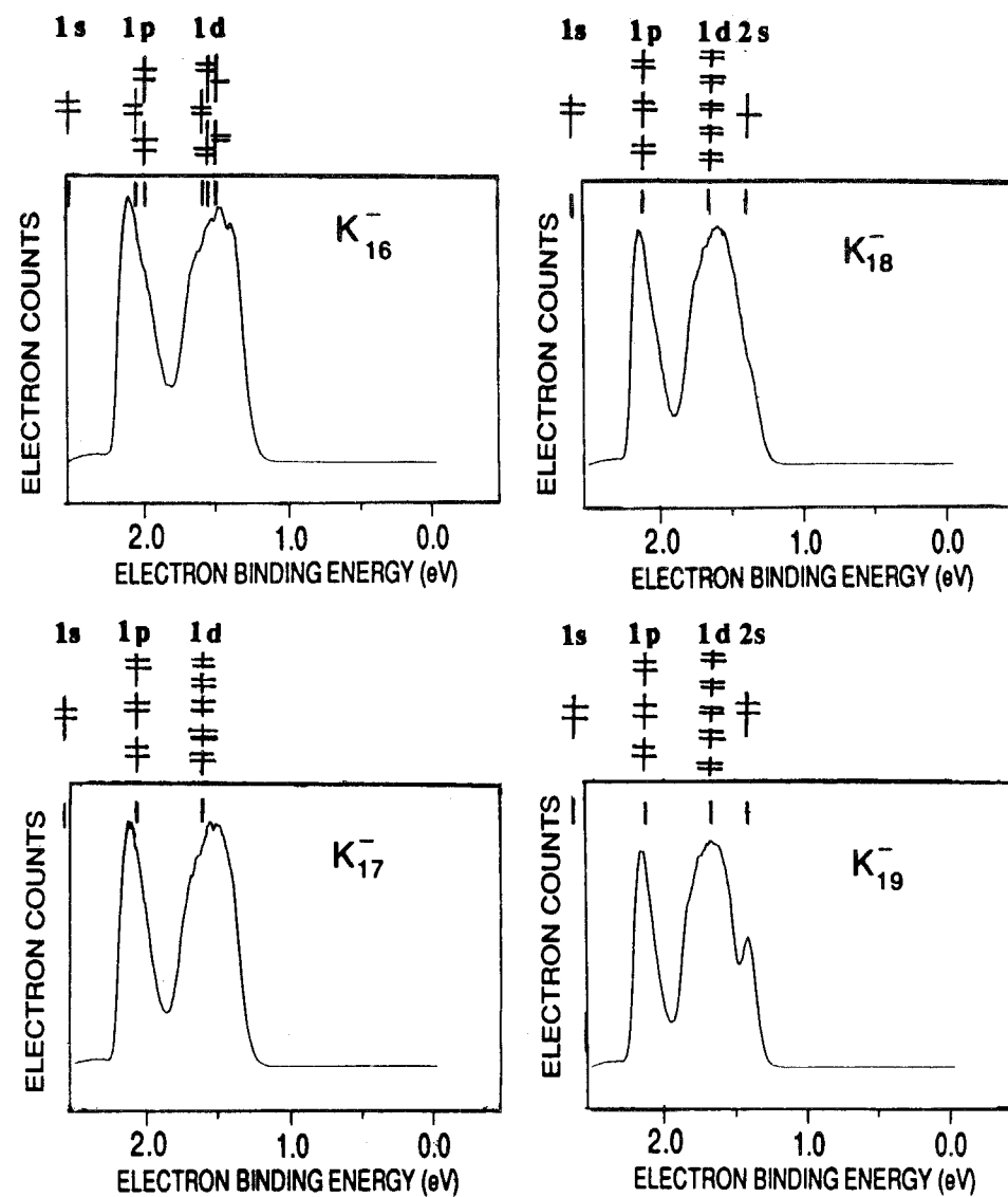
Figure 7. Comparisons of calculated shell model "stick spectra" with the corresponding observed photoelectron spectra of K_n^- ( n=16-19 ). The "stick spectra" are shown as insets on each photoelectron spectrum. Designations and electron occupations for individual levels are shown above each "stick spectrum".
