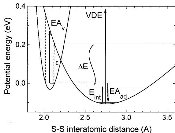
Figure 3. Sketch of the potential energy curves for the disulfide neutral and anion, as a function of the S-S bond length. In RETS experiments, electron attachment occurs, for a Rydberg electron energy \epsilon , and nascent excited anions are further stabilized by the Rydberg core during the collision by an energy amount of \Delta E slightly higher than \epsilon . Observed stable anions are those that are left with an internal energy E_{\text{int}} slightly lower than the adiabatic electron affinity EA_{\text{ad}} . See text for discussion.
