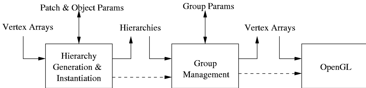
Figure 1: The GLOD object and dataflow model.
