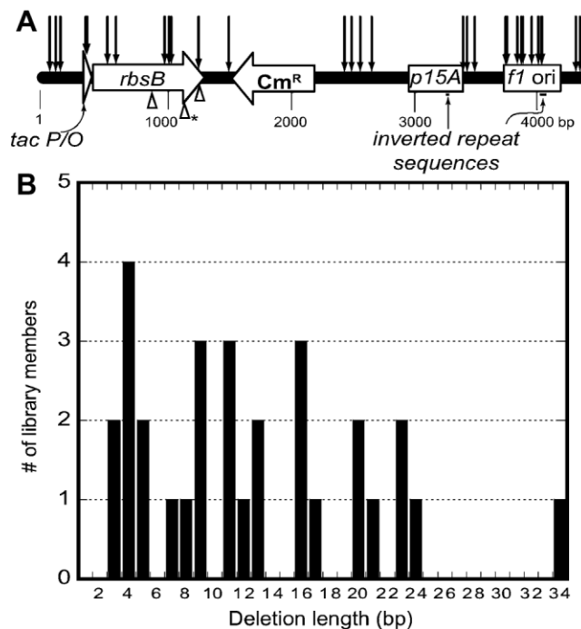
Figure 3. S1 nuclease digestion of supercoiled DNA results in a diverse set of products. A: To scale linear diagram of plasmid pDIMC8- rbsB with rbsB gene (including the rbsB signal sequence), tac promoter ( tacP/O ), p15A origin, f1 origin, and chloramphenicol resistance gene ( Cm R ) labeled. Arrows indicate the location of S1 nuclease digestion sites identified from sequencing of 30 naïve library members. Triangles indicate the location of S1 nuclease digestion sites in the switches discovered in the library, with four distinct switches discovered at the location marked by the asterisk. B: Distribution of deletion lengths at the site of S1 nuclease-created double stranded breaks in the same 30 naïve library members.
