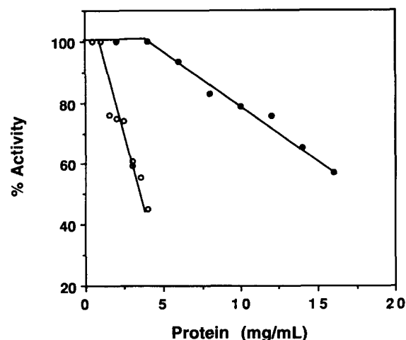
Fig. 2. Effect of protein concentration on the recovery of enzymatic activity of reduced TEM \beta -lactamase unfolded in 3 mM GdmCl for 3 h followed by removal of the denaturant by dialysis to a final denaturant concentration of 0.02 M. ●, 23 °C; ○, 37 °C.
