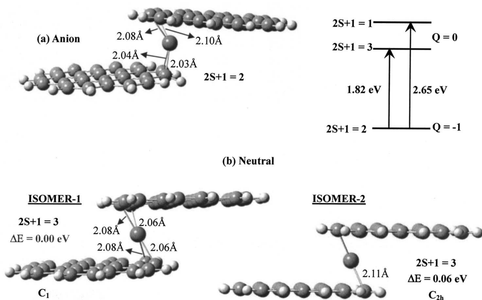
FIG. 6. (a) The ground state isomer of the negatively charged \text{Fe}_1(\text{coronene})_2^- complex. (b) The ground state and the next higher energy isomer of the neutral \text{Fe}_1(\text{coronene})_2 complex. The calculated photodetachment transition energies for the ground state anion are also shown.
