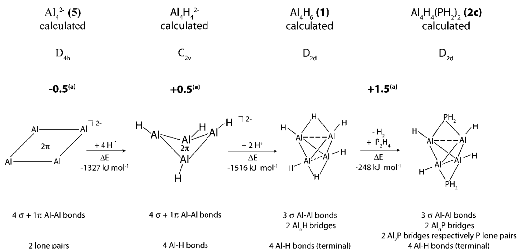
Scheme 2. Energetic Relations and Relations with Respect to Number and Kind of Bonds in the Species \text{Al}_4^{2-} ( 5 ), \text{Al}_4\text{H}_4^{2-} , \text{Al}_4\text{H}_6 ( 1 ), and \text{Al}_4\text{H}_4(\text{PH}_2)_2 ( 2c )
