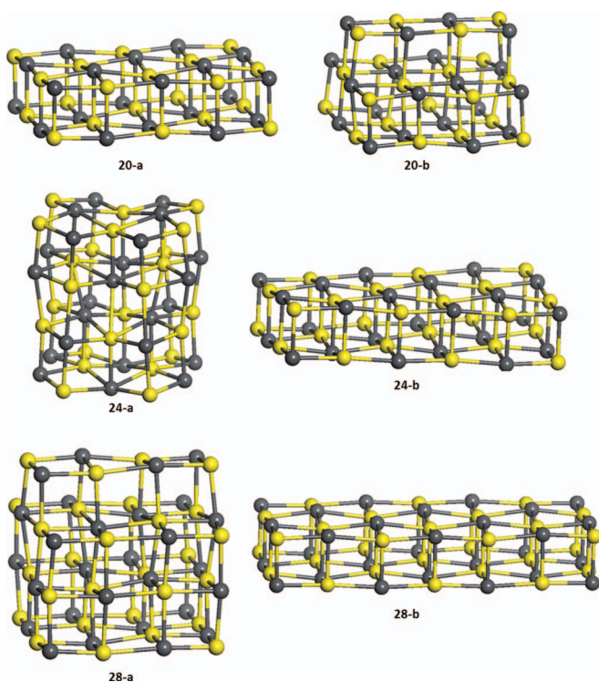
FIG. 2. Structures of lowest, (a), and higher, (b), energy isomers of (\text{PbS})_{4n} ( n = 5, 6, \text{ and } 7 ).
